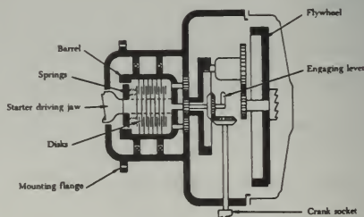
FIGURE 5-3. Torque overload release clutch.
